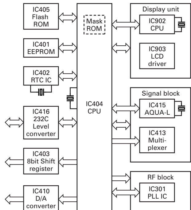
Fig. 5 Control circuit block diagram
