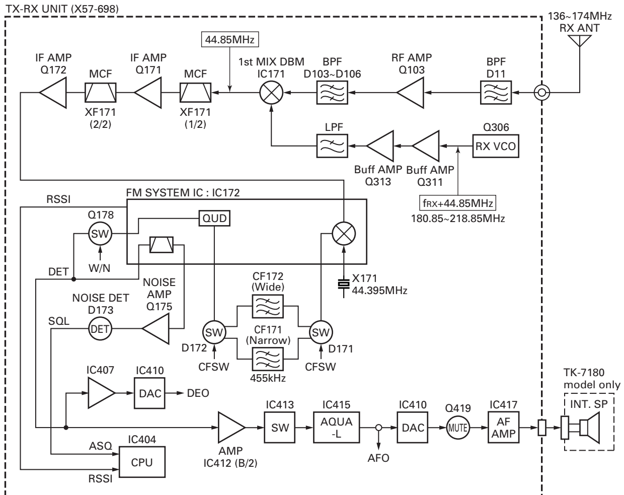
Fig. 1 Receiver circuit
