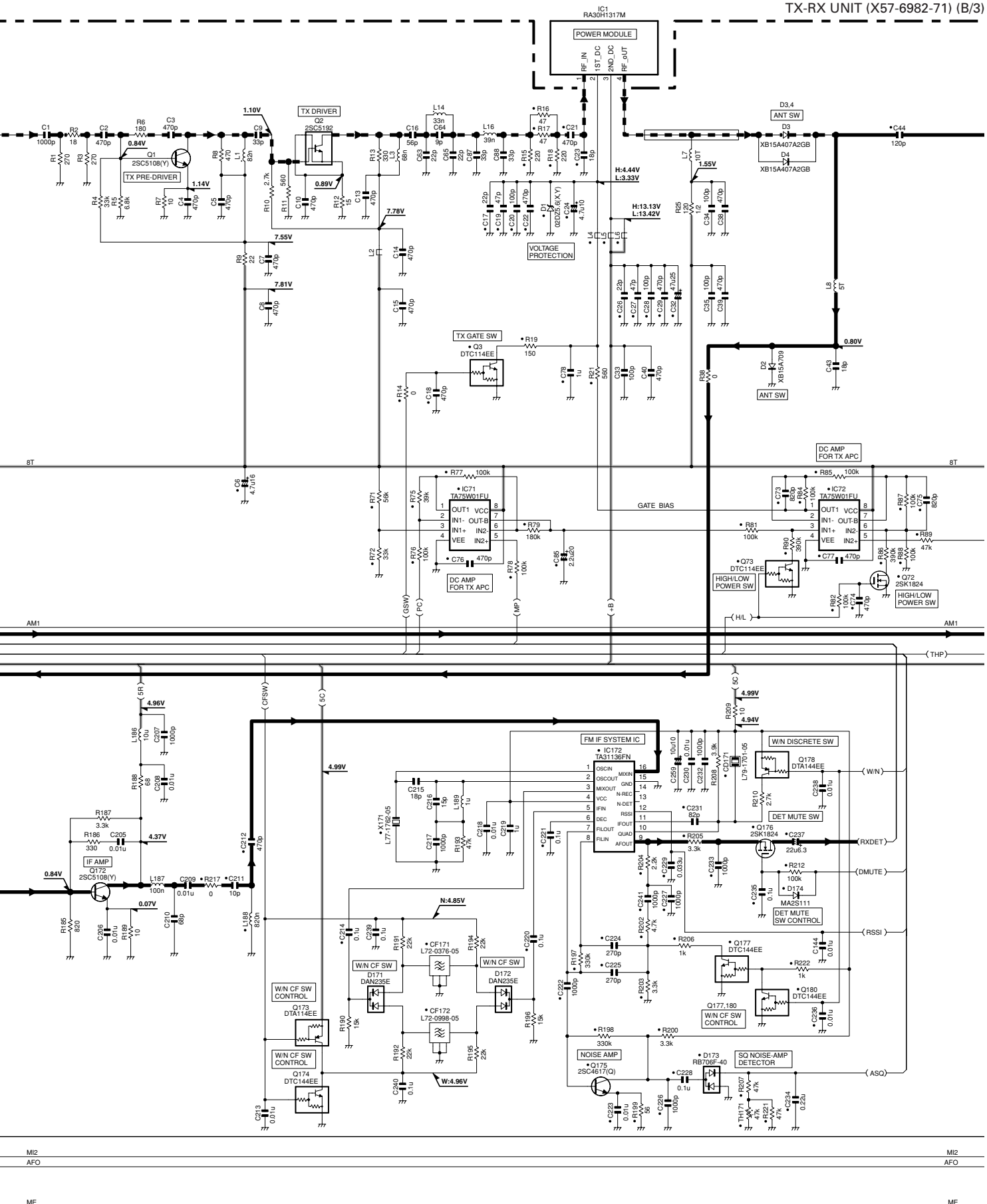
TX-RX UNIT (X57-6982-71) (B/3)
