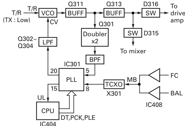
Fig. 4 PLL block diagram
