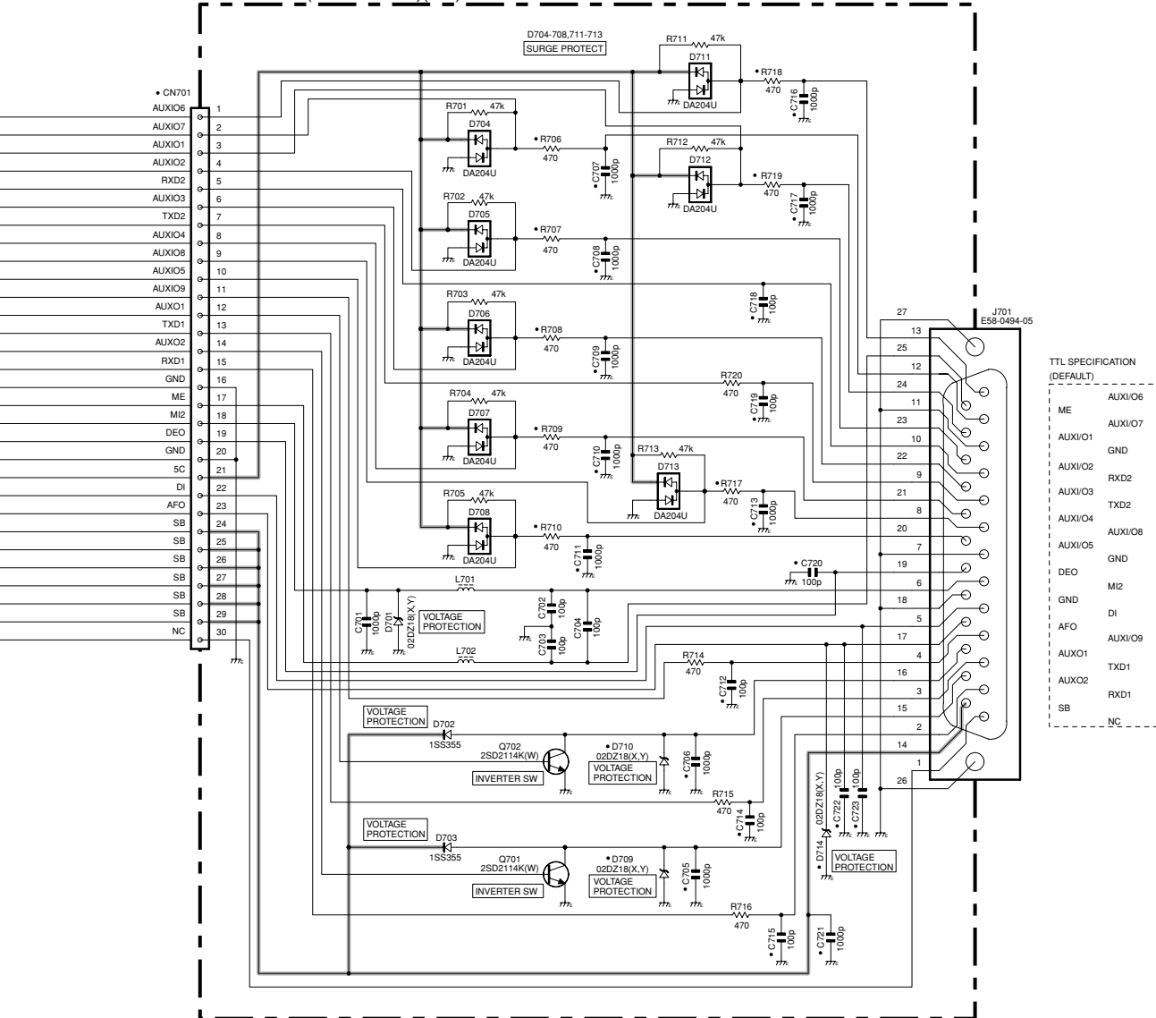
TX-RX UNIT (X57-6982-71)(A/3)
